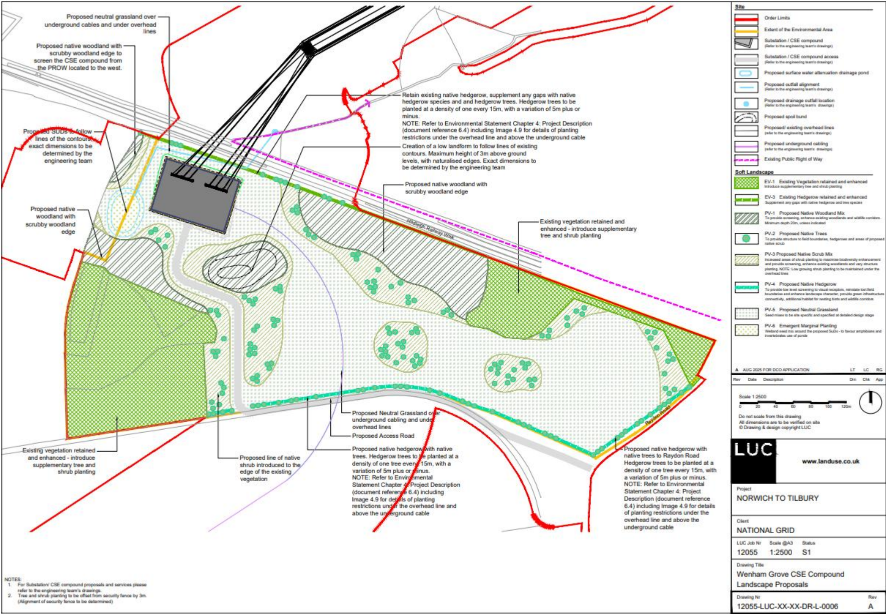
Image 1.2 Wenham Grove CSE Compound (Source: Appendix D of the Outline LEMP (Revision A))
