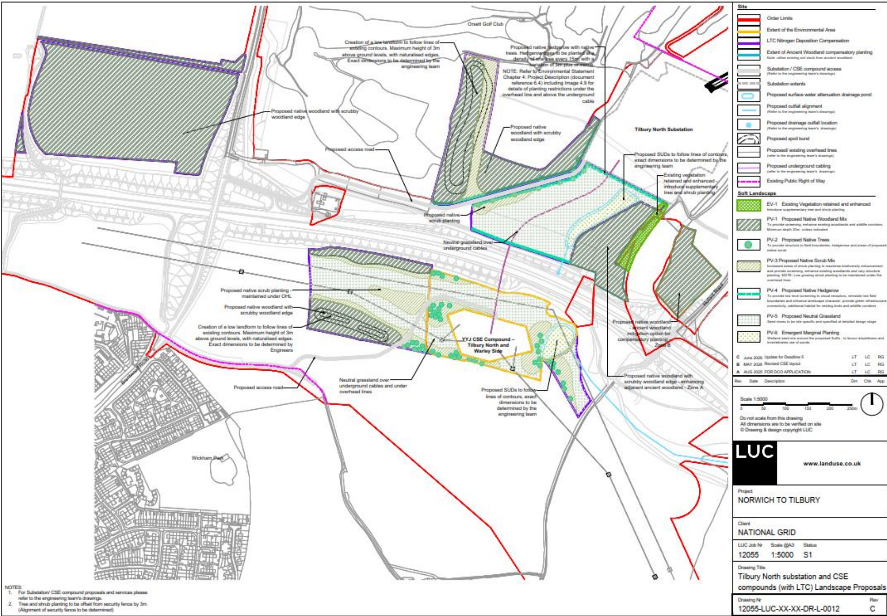
Image 1.6 Tilbury North (YYJ) CSE Compound (Tilbury North and Warley Side) and Tilbury North Substation with Lower Thames Crossing mitigation (Source: Appendix D of the Outline LEMP (Revision C))
